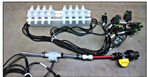
Flowmeters w/ Hose barb fittings and bracket
